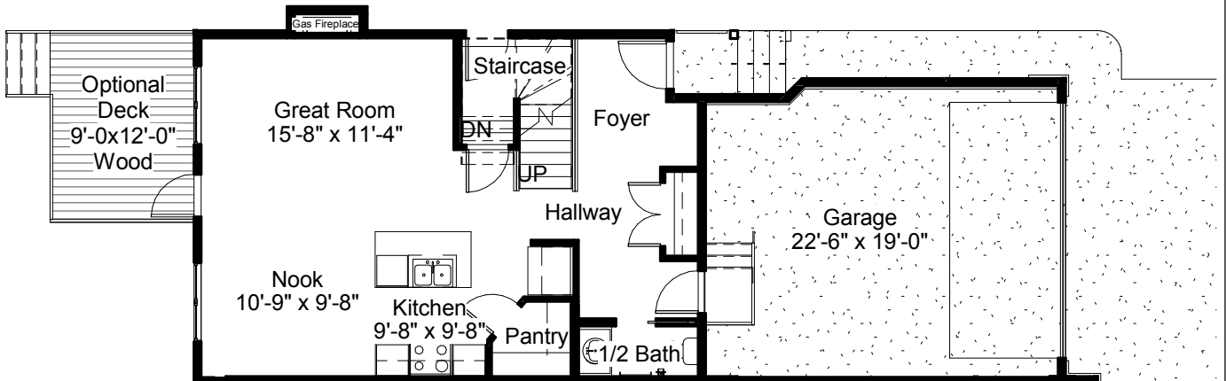
Unit 1B Main Floor Plan 9'-1" Main Floor Ceiling
