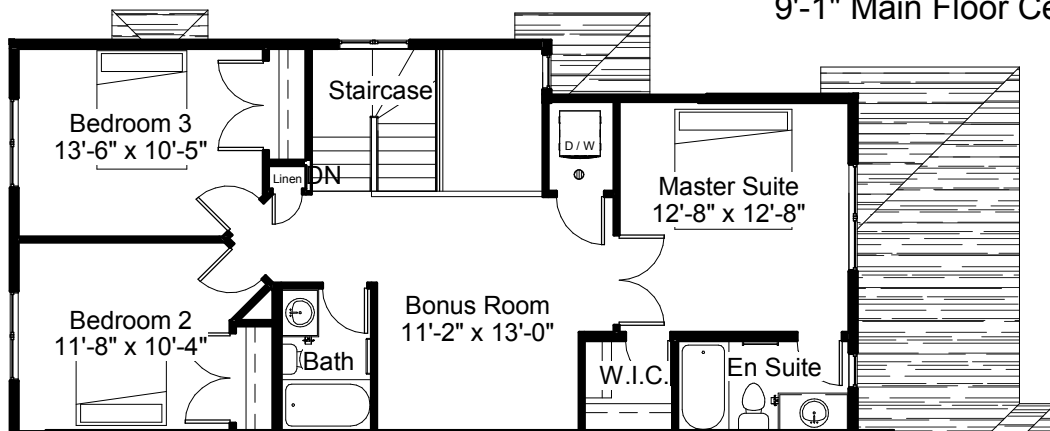
Unit 1B Second Floor Plan 8'-1" Second Floor Ceiling
