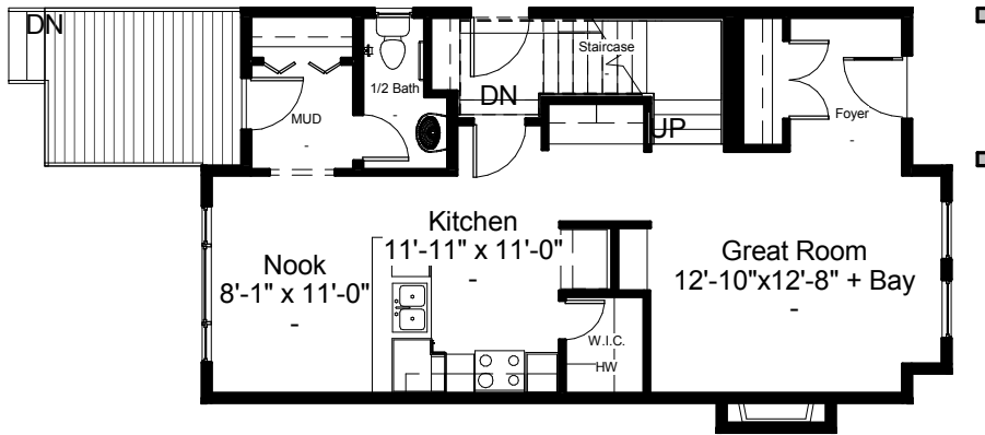
Main Floor Plan 725 SQFT 8'-1" Main Floor Ceiling
