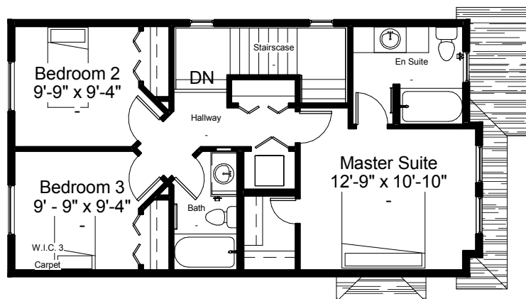
Second Floor Plan 731 SQFT 8'-1" Second Floor Ceiling
