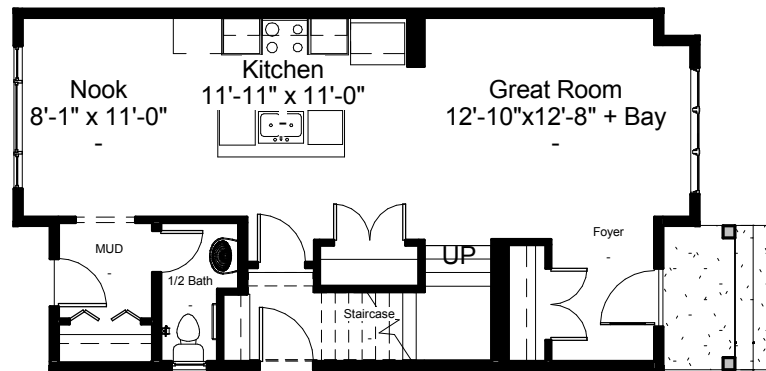
Main Floor Plan 725 SQFT 8'-1" Main Floor Ceiling
