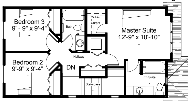
Second Floor Plan 731 SQFT 8'-1" Second Floor Ceiling
