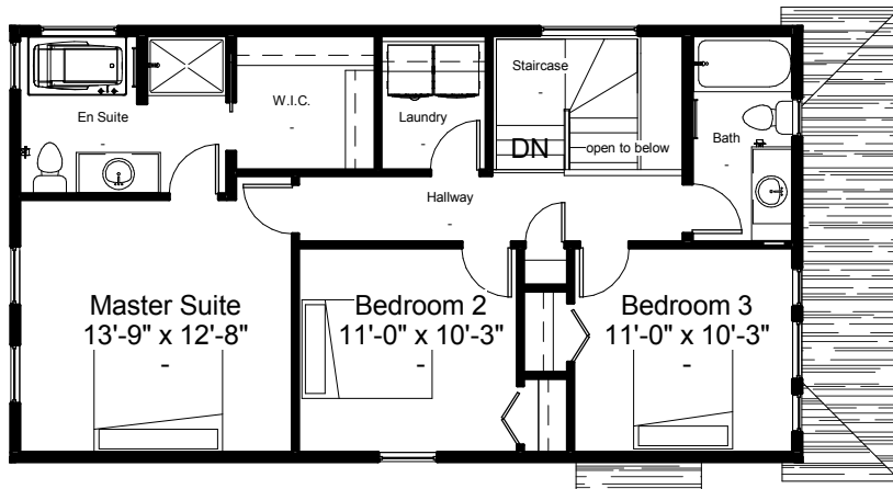
Second Floor Plan 880 SQFT 8'-1" Second Floor Ceiling
