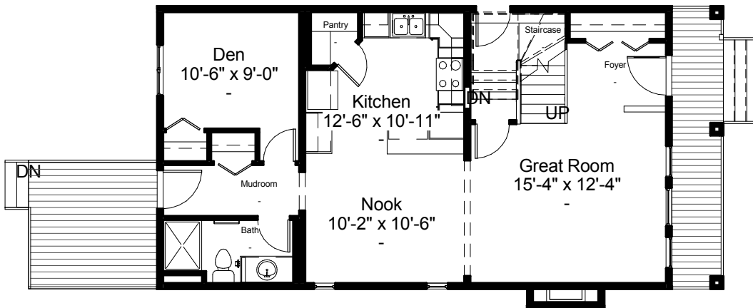
Main Floor Plan 880 SQFT 8'-1" Main Floor Ceiling
