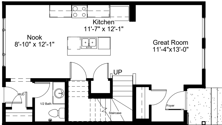
Main Floor Plan 642 SQFT 9'-1" Main Floor Ceiling
