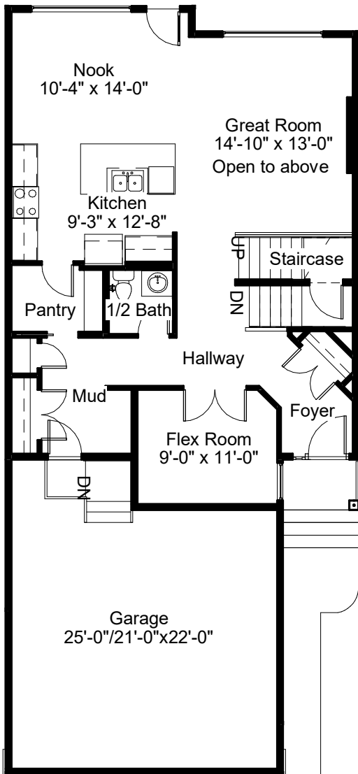
Main Floor Plan - 1029 SQFT 9'-1" Main Floor Ceiling
