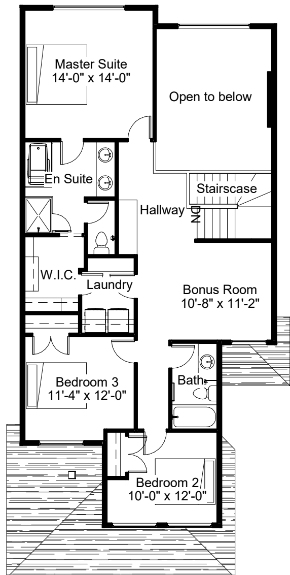
Second Floor Plan 1160 SQFT 8'-1" Second Floor Ceiling
