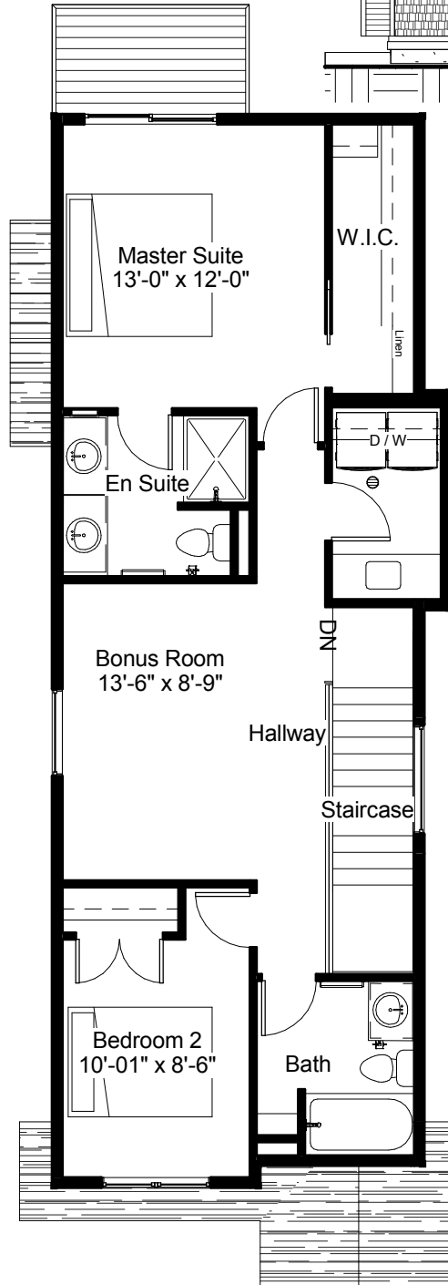
Second Floor Plan - 769 SQFT 8'-1" Second Floor Ceiling
