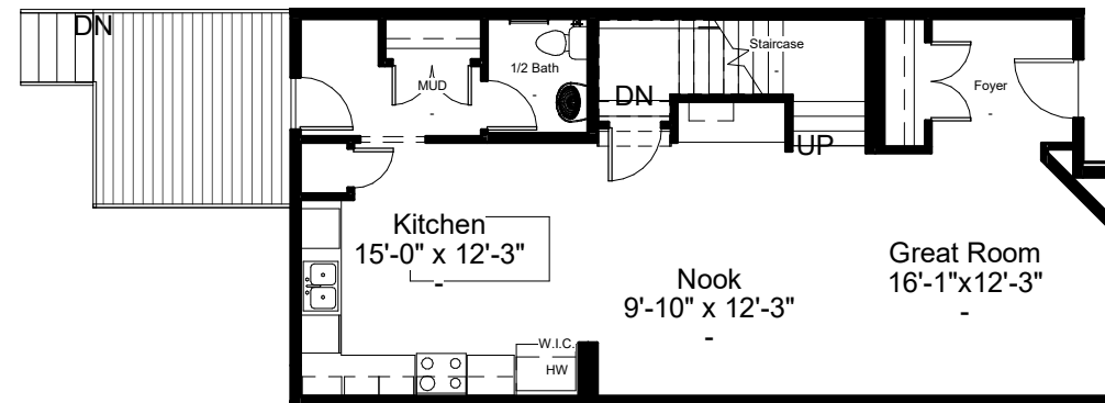
Main Floor Plan 824 SQFT 9'-1" Main Floor Ceiling
