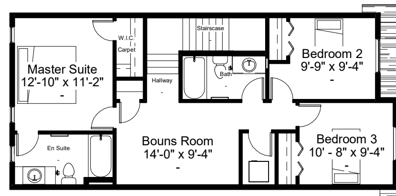
Second Floor Plan 861 SQFT 8'-1" Second Floor Ceiling
